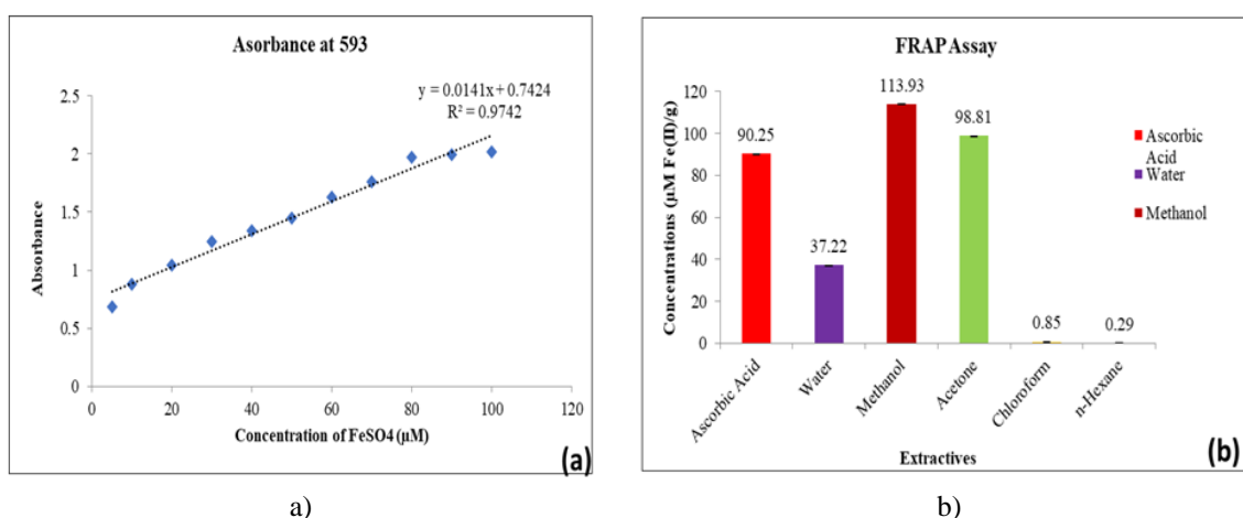
Figure 2. FRAP Assay. a) Standard curve for FeSO 4 , b) concentrations for the total antioxidant present in different solvent
