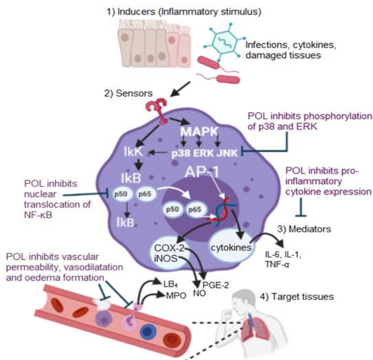
Figure 2. Molecular mechanisms of the anti-inflammatory effect of POL. NF- \kappa B is a family of dimeric transcription factors that includes five protein monomers (p65, RelB, cRel, p50, and p52). Activation of NF- \kappa B starts with the degradation of I \kappa B inhibitor proteins allowing nuclear translocation of free NF- \kappa B dimer (e.g., p50-p65). Activating Protein 1 (AP-1) is a transcription factor composed mainly of proteins belonging to the c-Jun and c-Fos families and is also related to the regulation of genes involved in inflammation.
