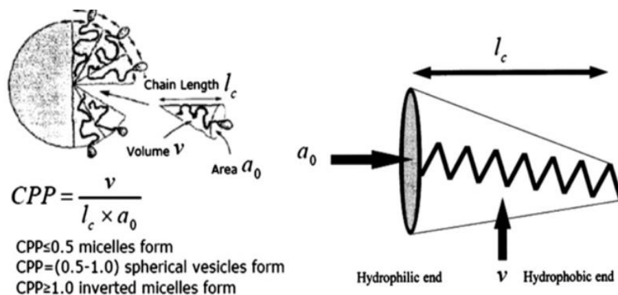
Figure 3. Critical packing parameter of an amphiphile.
