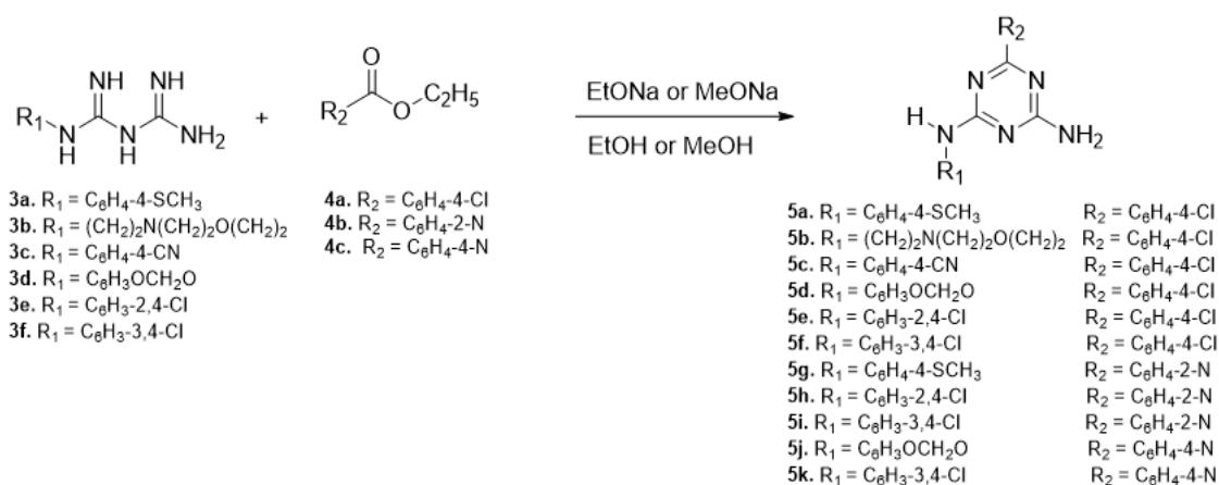
Scheme 2. Synthesis of 6-aryl-2,4-diamino-1,3,5-triazines
